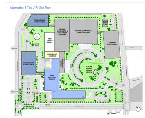
Figure 3. Alternative A - Site Layout.
